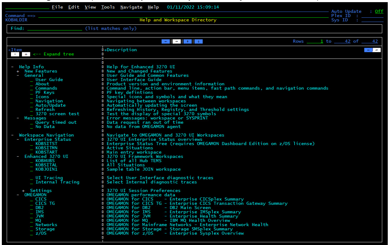
Figure 3. Help Tree.
